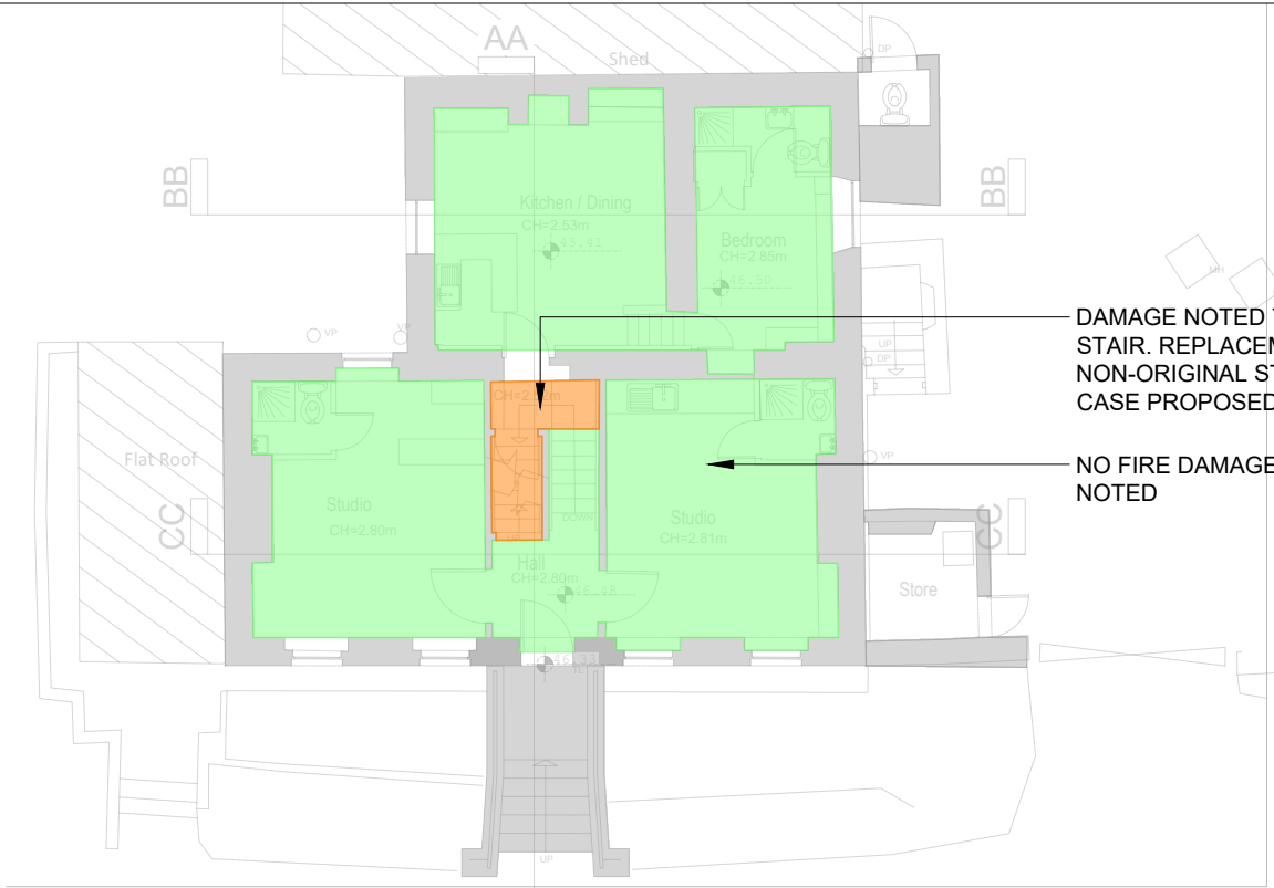
UPPER GROUND FLOOR PLAN SCALE 1:150
