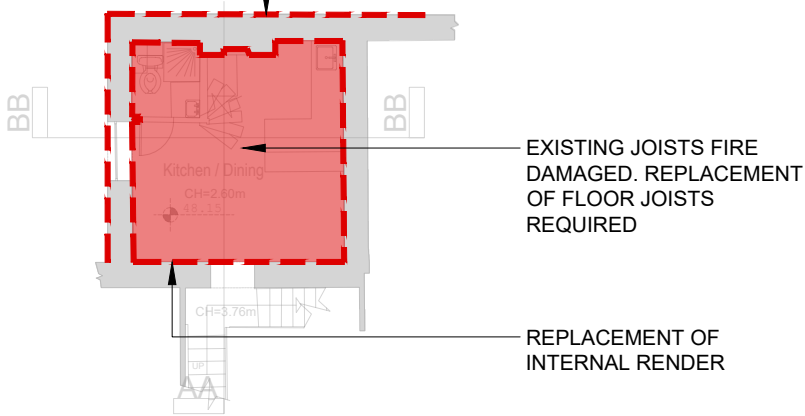
LOWER GROUND FLOOR PLAN SCALE 1:150
