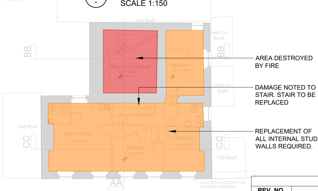
UPPER GROUND FLOOR PLAN SCALE 1:150
