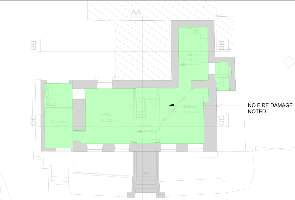
LOWER GROUND FLOOR PLAN SCALE 1:150
